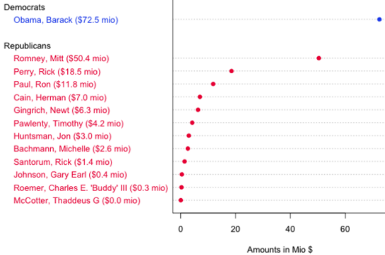
Figure 75. visualizations to spot underlying patterns (Gregor Aisch)
