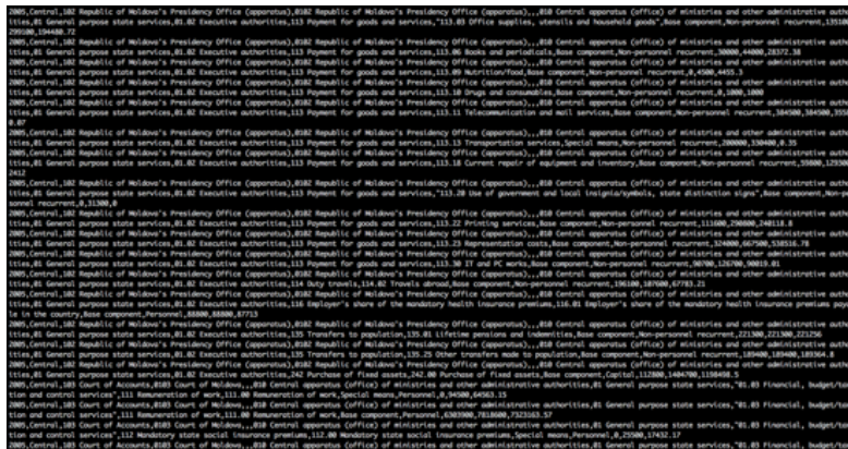
Figure 69. Messy Data
