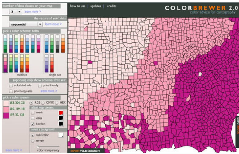
Figure 108. Color brewer
