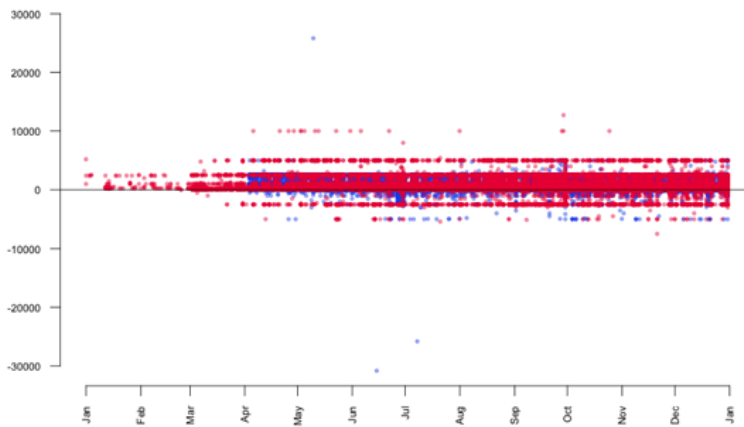
Figure 77. Removing the outliers (Gregor Aisch)
